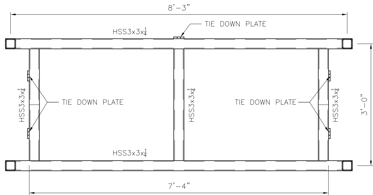
3 LIFT FRAME BOTTOM SKID 1" = 1'-0"
