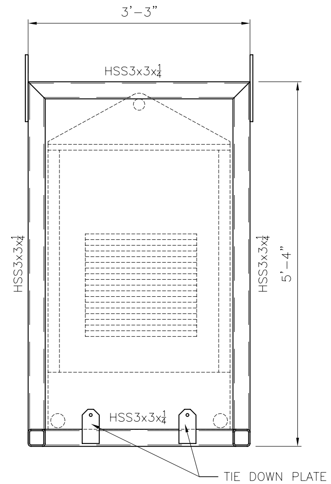
2 LIFT FRAME END ELEVATION 1" = 1'-0"
