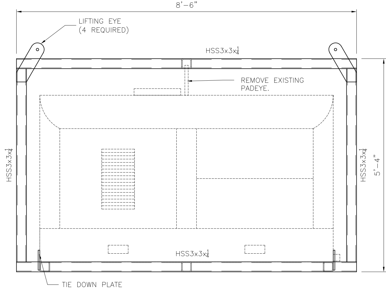
1 LIFT FRAME SIDE ELEVATION 1" = 1'-0"
